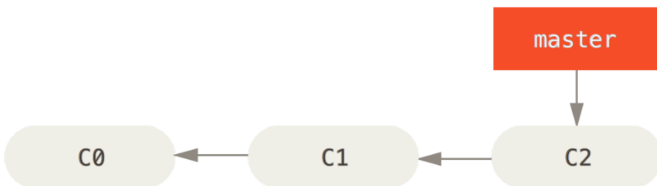
Figure 18. A simple commit history
